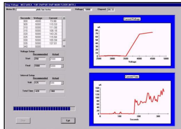
Figure 14. Failed Insulation System
