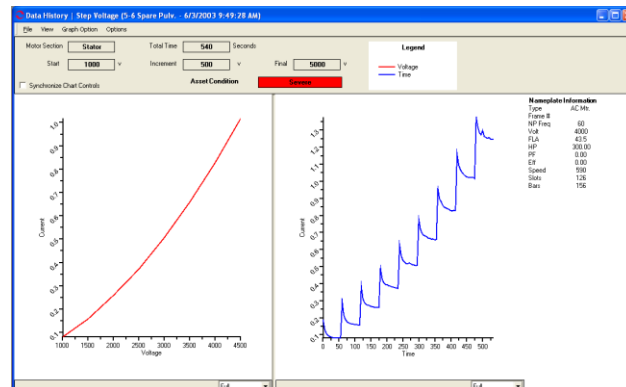
Figure 13. Step Voltage Test
