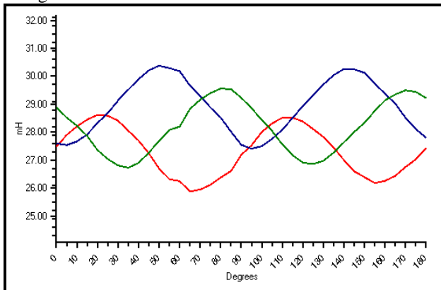
Figure 25. Concentric Wound Motor RIC Graph
